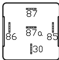
High Beam Drivers Side Relay
