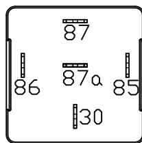
Low Beam Drivers Side Relay
