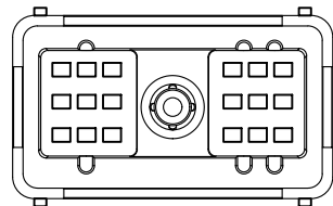
PIN FACE FRONT VIEW
